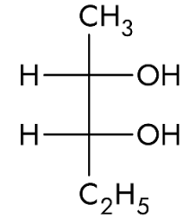
(2R,3S)-pentano-2,3-diol
