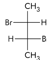
(2R,3R)-2,3-dibromobutan
