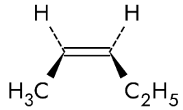
(2Z)-pent-2-en
