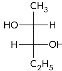
(2R,3R)-pentano-2,3-diol
