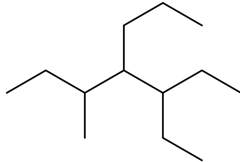
3-etylo-5-metylo-4-propyloheptan
