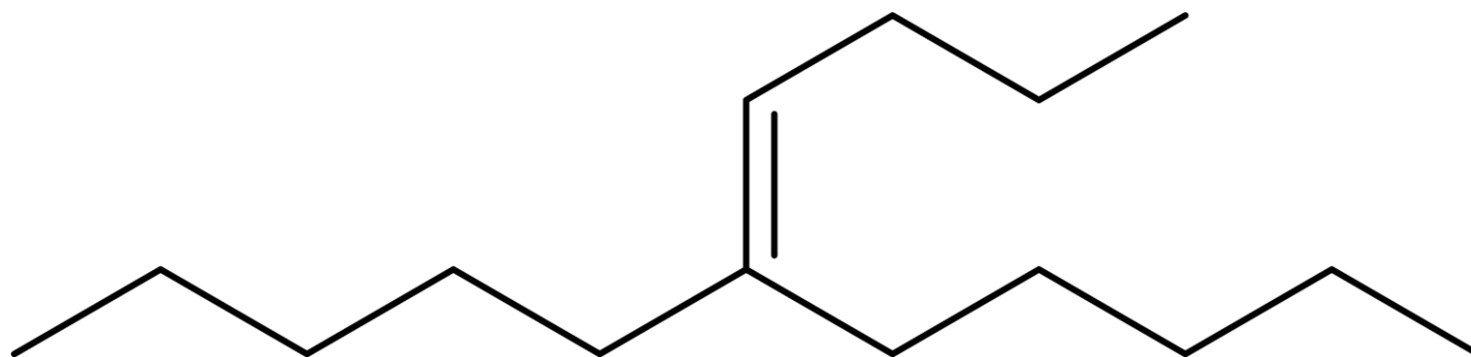
6-butylidenoundekan
