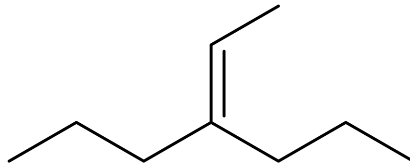
4-etylidenheptan
