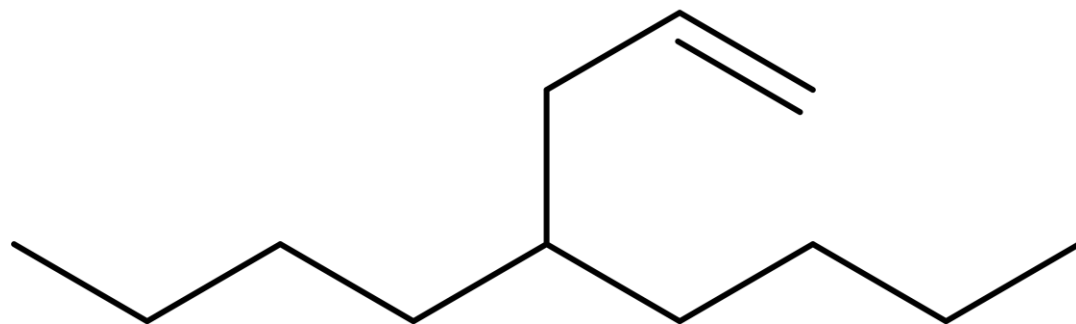
5-(prop-2-en-1-ylo)nonan
