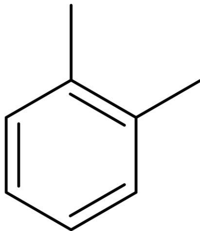
1,2-dimetylobenzen
