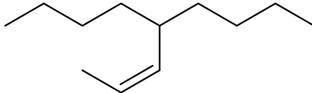
5-(prop-1-en-1-ylo)nonan
