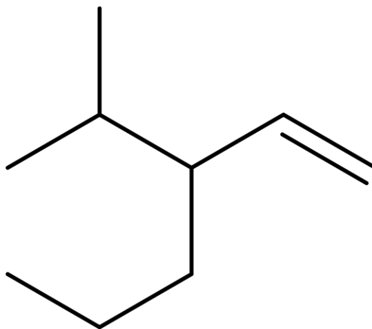
3-(prop-2-ylo)heks-1-en
