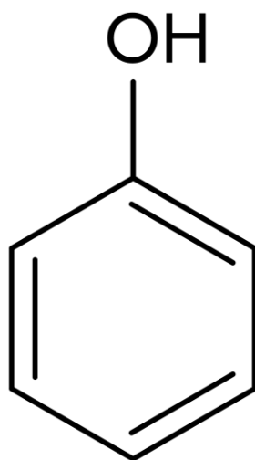
fenol
