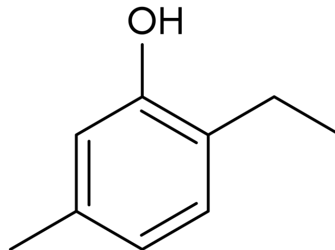
2-etylo-5-metylofenol
