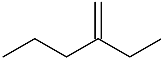
3-metylidenohexsan
