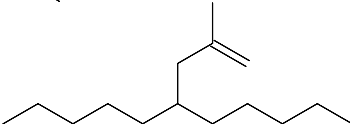
6-(2-metyloprop-2-en-1-yl)undekan
