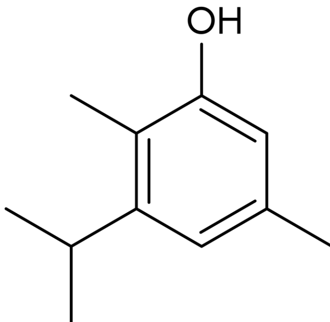
5-etylo-2-metylo-3-(prop-2-ylo)fenol
