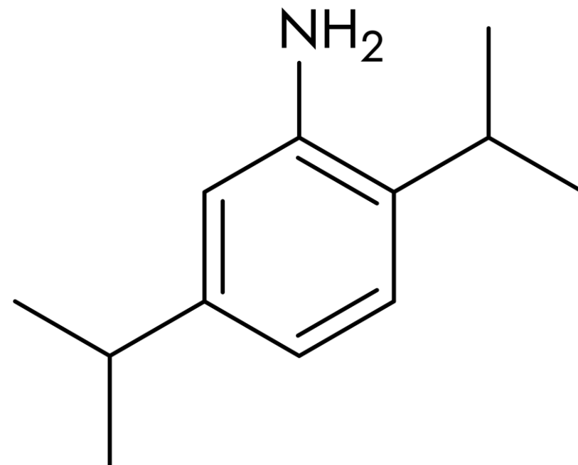
2,5-di(propan-2-ylo)anilina
