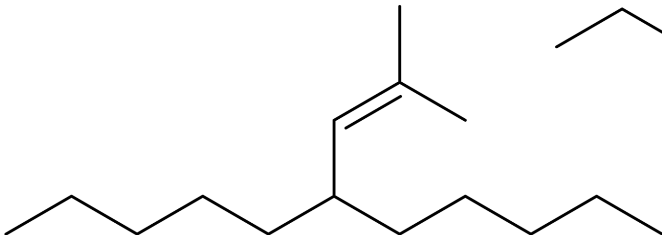
6-(2-metyloprop-1-en-1-yl)undekan
