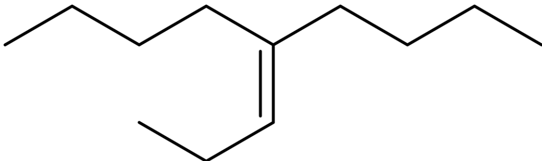
5-propylidenononan
